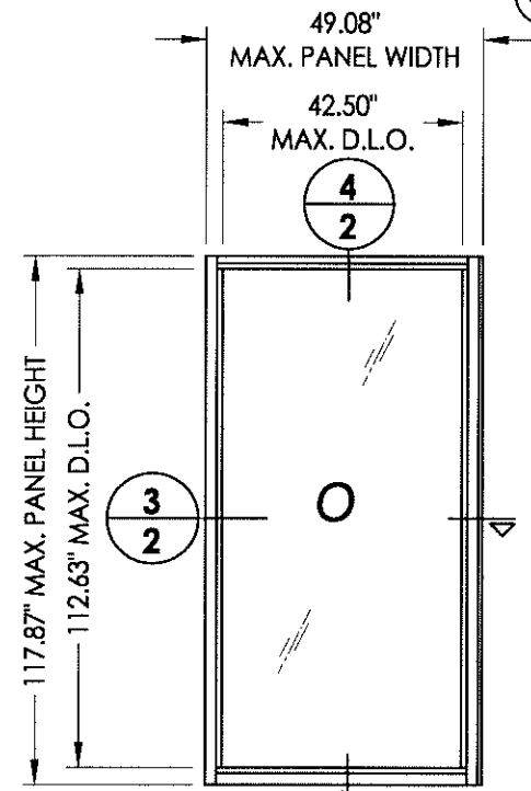
FIXED PANEL
