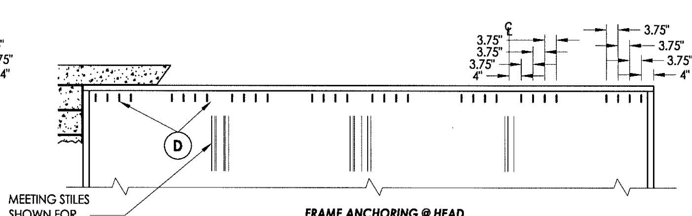
FRAME ANCHORING @ HEAD DP <= 100 PSF Max. shim space <= .25"
