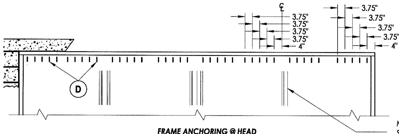
FRAME ANCHORING @ HEAD DP <= 70 PSF Max. shim space <= .625"
