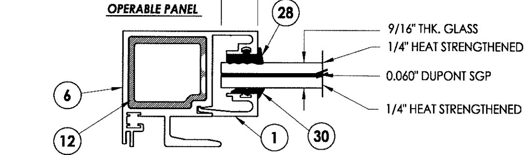
G2 GLAZING DETAIL (DRY GLAZED) MONOLITHIC 9/16\"/>
