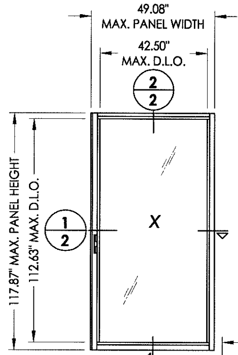
OPERABLE PANEL
