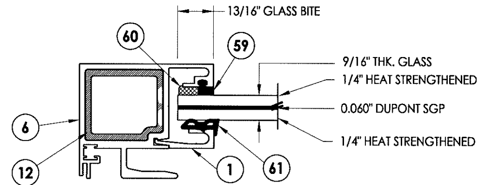
G3 GLAZING DETAIL (WET GLAZED) MONOLITHIC 9/16\"/>
