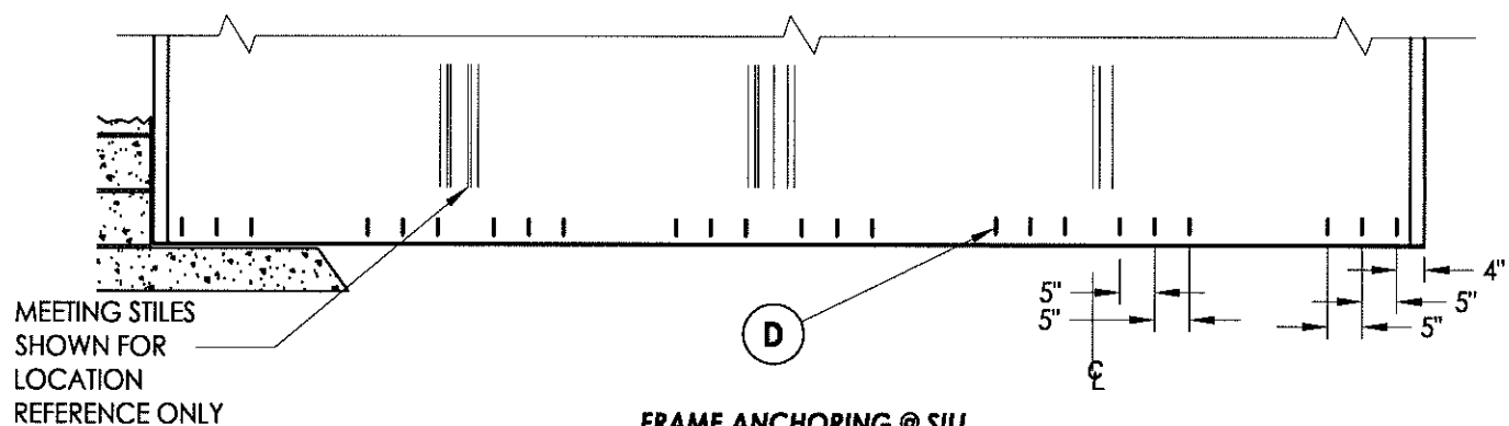
FRAME ANCHORING @ SILL DP <= 100 PSF Max. shim space <= 0.17"
